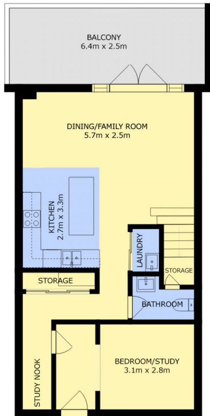
FLOOR 1
