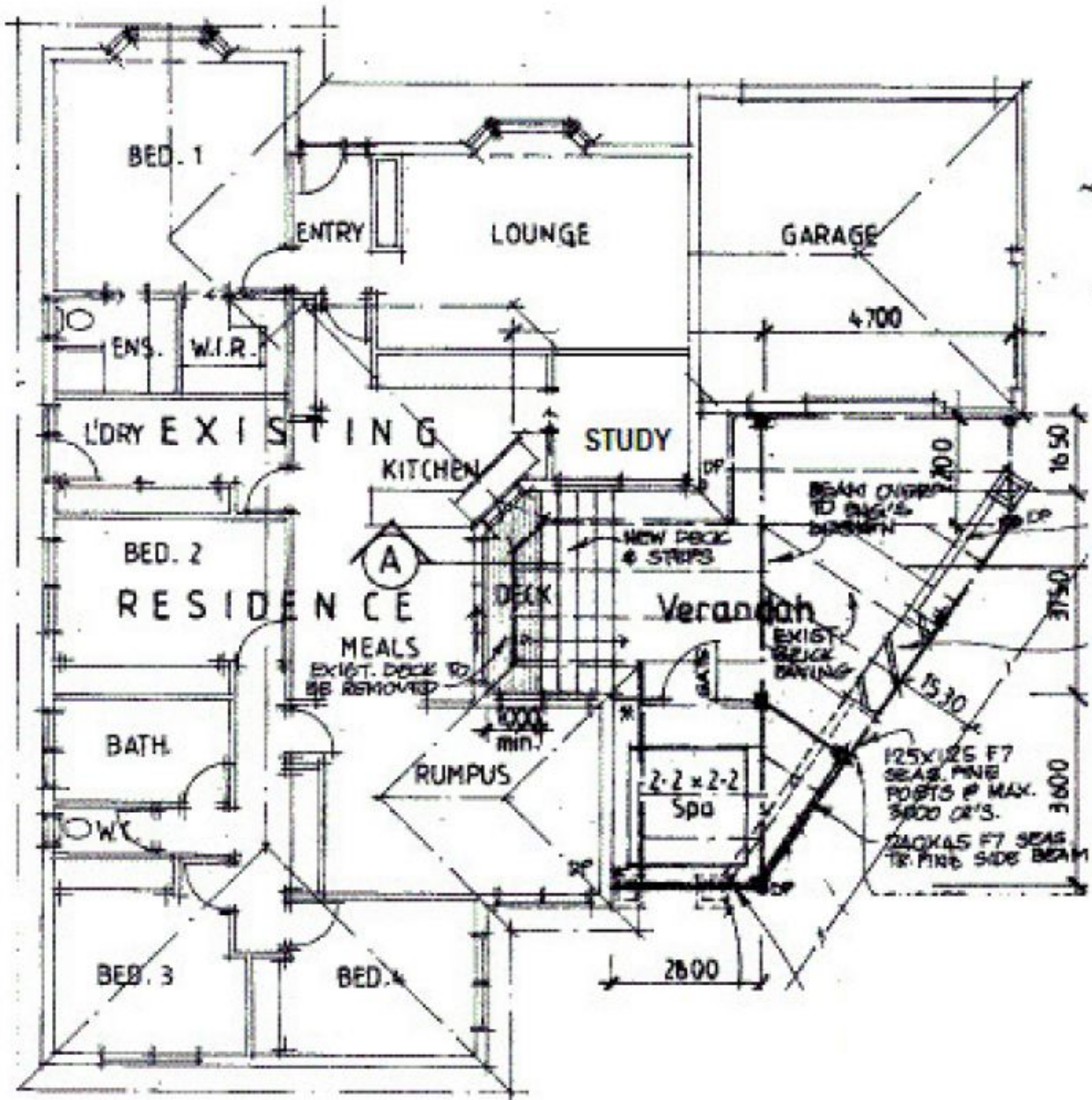
FLOOR PLAN
