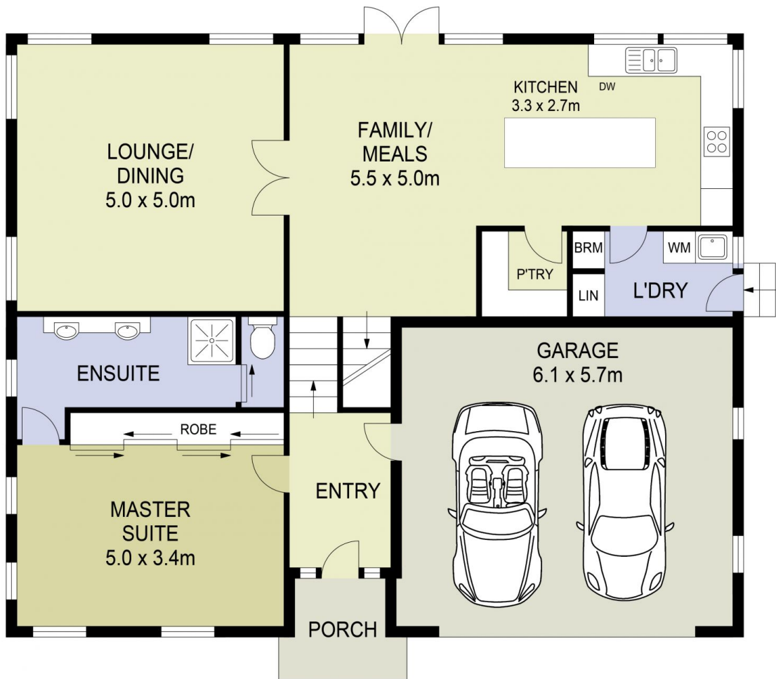
GROUND FLOOR
