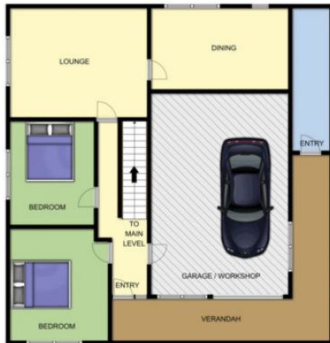
LOWER LEVEL
