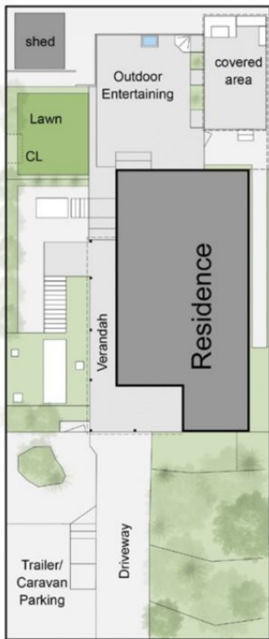
Site Plan
