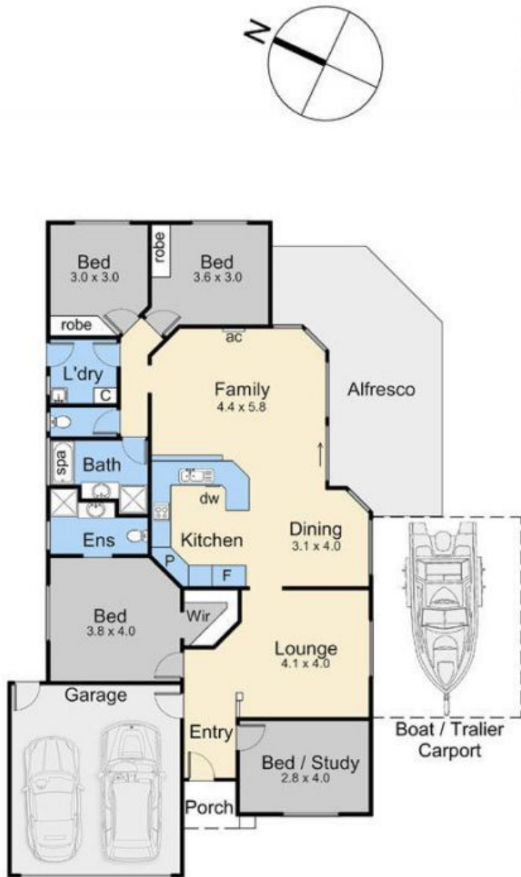
Floor Plan
