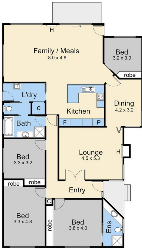
Floor Plan
