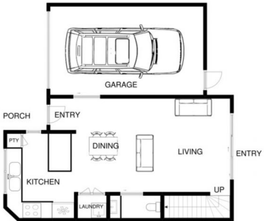
MAIN LEVEL
