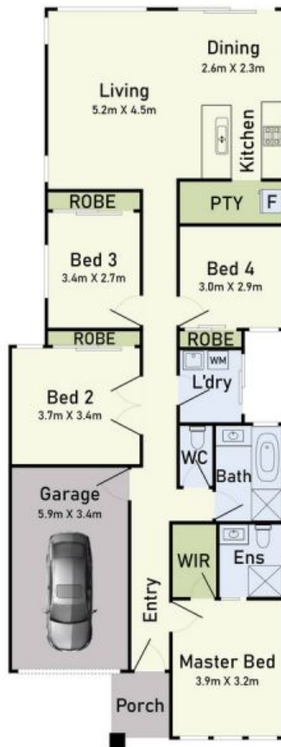
Floor Plan
