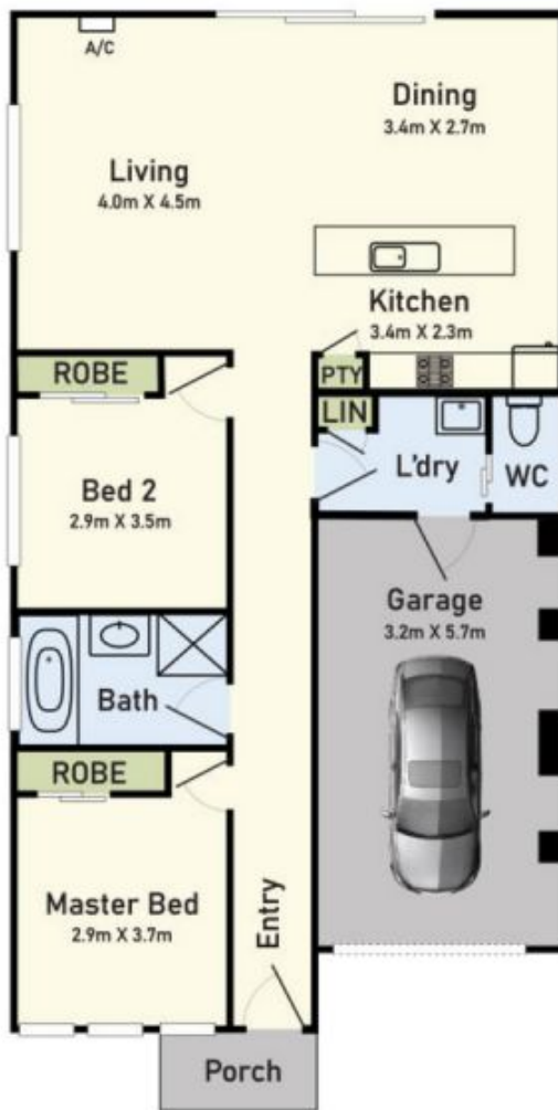
Floor Plan
