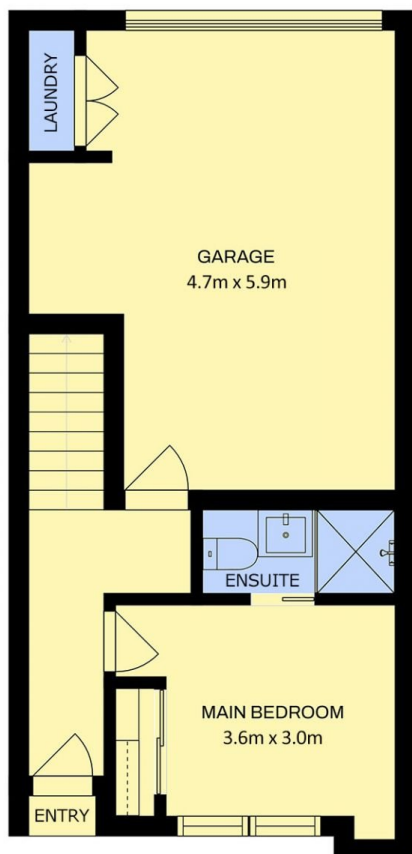
FLOOR 1
